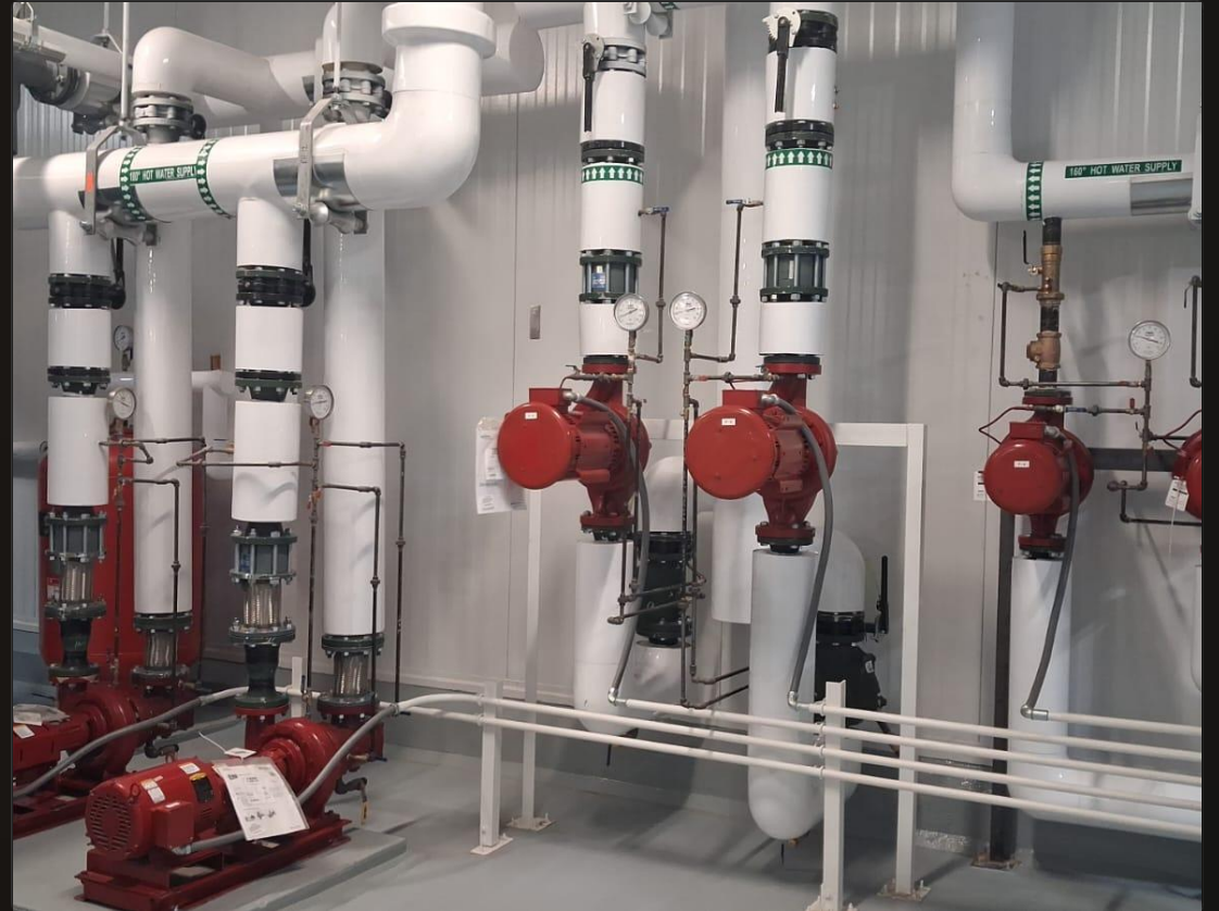
SANITARY STAINLESS STEEL INSTALATIONS
